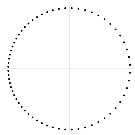
FIGURE 1. A schematic figure of the solutions to (2.21–2.22) giving the approximate locations of partition function zeros of the Ising model in parameter z which is related to the external field h by z = e^{2h} . The plot corresponds to dimension d = 2 and torus side L = 8 . The expansion used for calculating the quantities \zeta_{\pm} is shown in (2.23). To make the non-uniformity of the spacing between zeros more apparent, the plot has been rendered for the choice e^{2J} = 2.5 even though this is beyond the region where we can prove convergence of our expansions.
